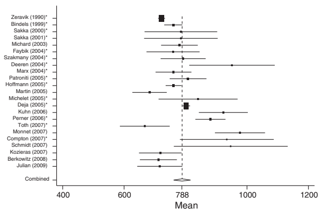
Figure 5 Forest plot of individual study results and pooled mean estimator from a random-effects meta analysis concerning GEDVI data in non-surgical patients (SEP). *Studies in which ITBVI was transformed to GEDVI ( GEDVI = ITBVI/1.25 ).
