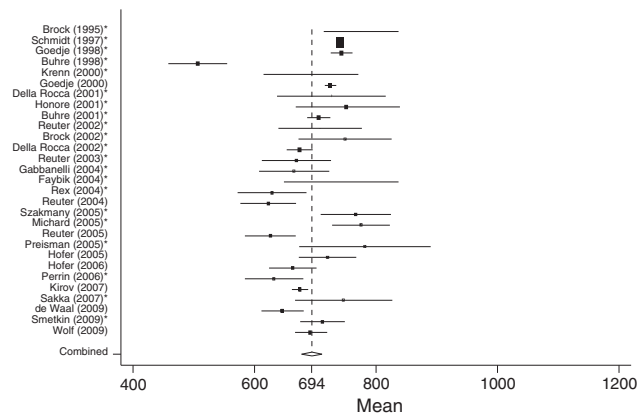
Figure 4 Forest plot of individual study results and pooled mean estimator from a random-effects meta analysis concerning GEDVI data in surgical patients (SURG). *Studies in which ITBVI was transformed to GEDVI ( GEDVI = ITBVI/1.25 ).
