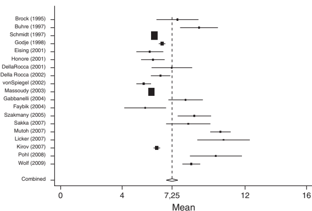
Figure 6 Forest plot of individual study results and pooled mean estimator from a random-effects meta analysis concerning EVLWI data in surgical patients (SURG).
