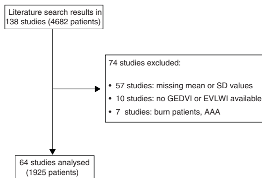
Figure 3 Flow of study inclusion. SD = standard deviation, GEDVI = global end-diastolic volume index, EVLWI = extravascular lung water index, AAA = aortic aneurysm repair including aortic clamping and axillary catheterization.
